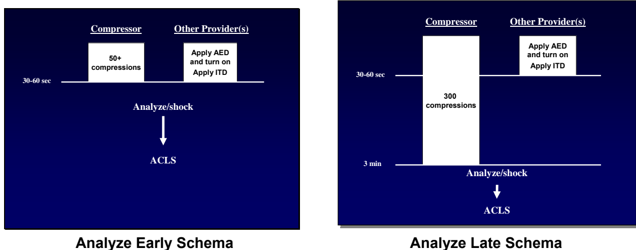
Figure 5: Training Scheme
