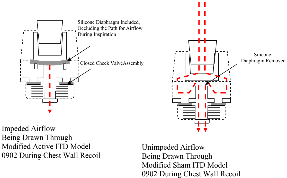
Figure 3. Airflow through Active and Sham ITD during Decompression (Chest Wall Recoil)
