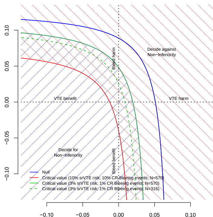
Figure 2: Bivariate decision criteria.
