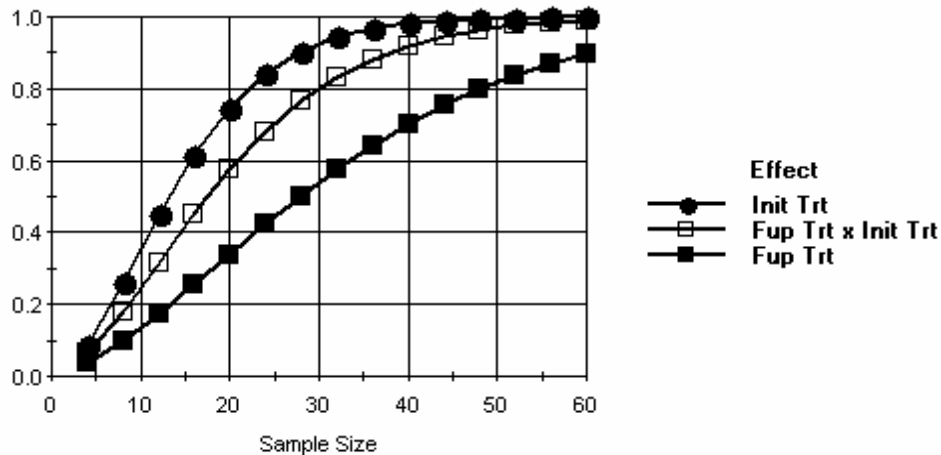
Figure 4.3* Power of a 2 X 2 Factorial as a Function of Per-Cell Sample size
